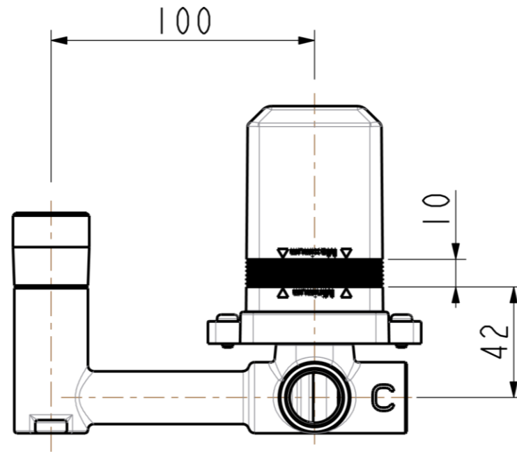
In-wall Assembly
