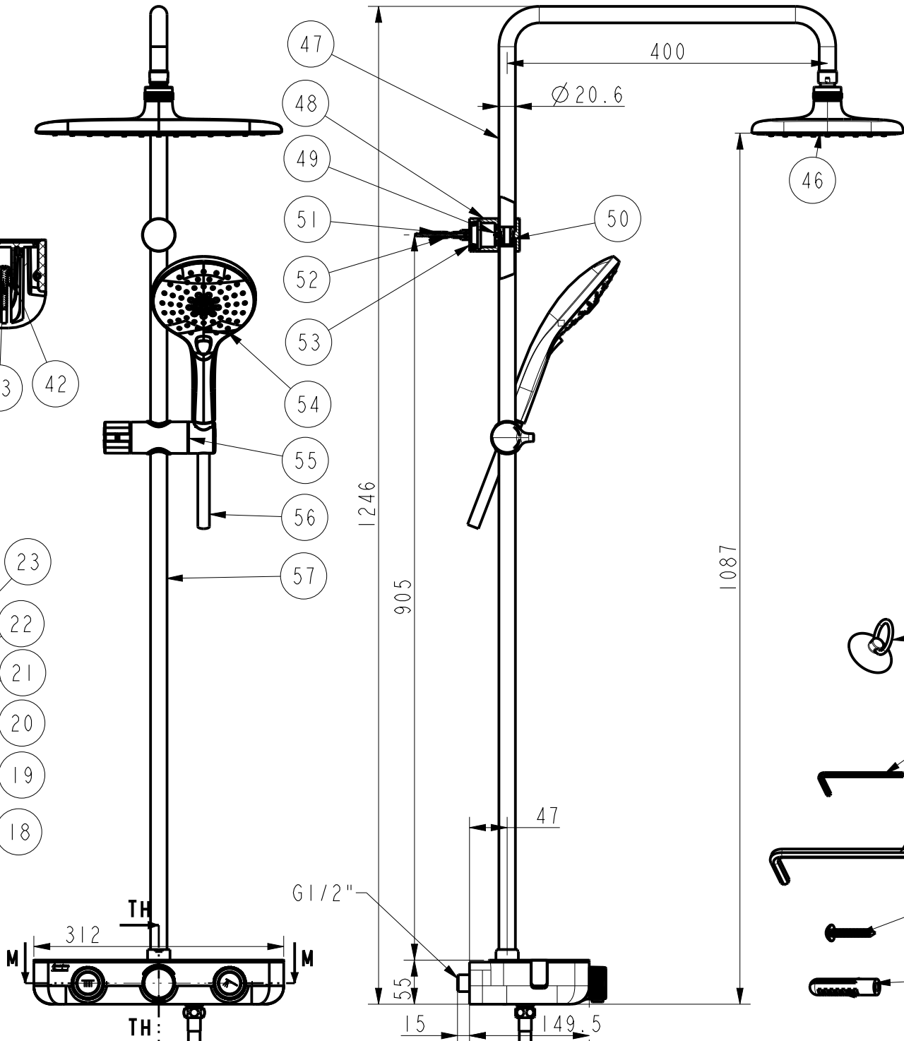
SECTION TH-TH
