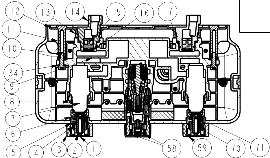
SECTION M-M SCALE 0.300
