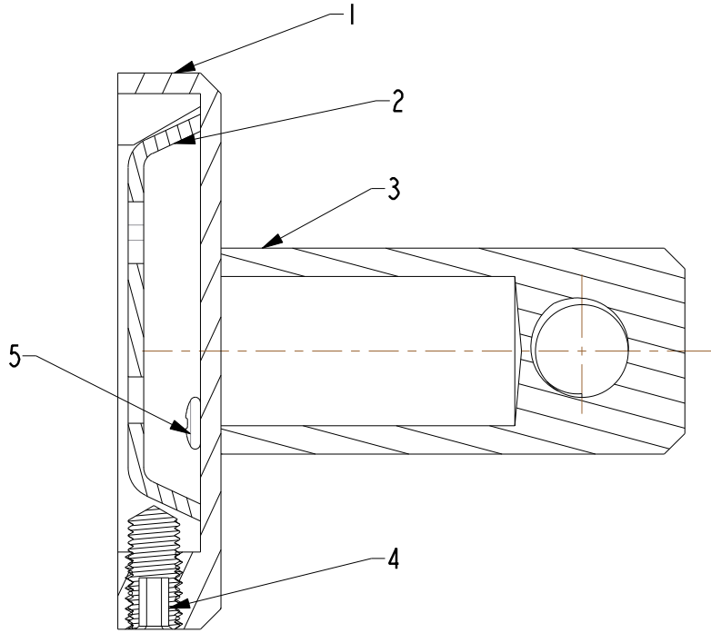
SECTION C-C
