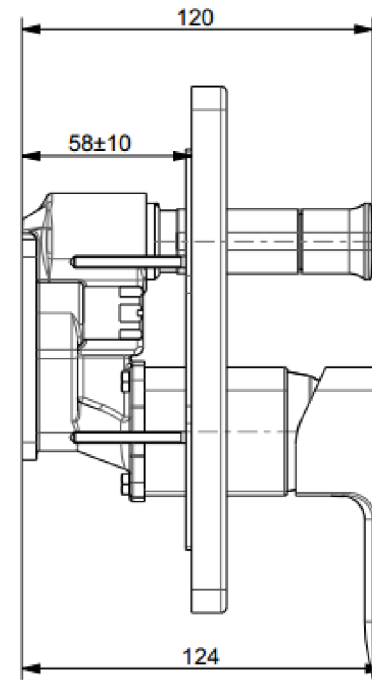
The installation of hollow wall
