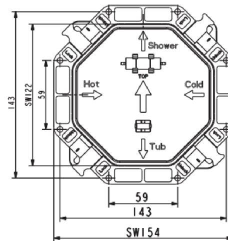
The installation of hollow wall
