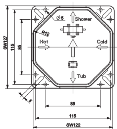
The installation of solid wall
