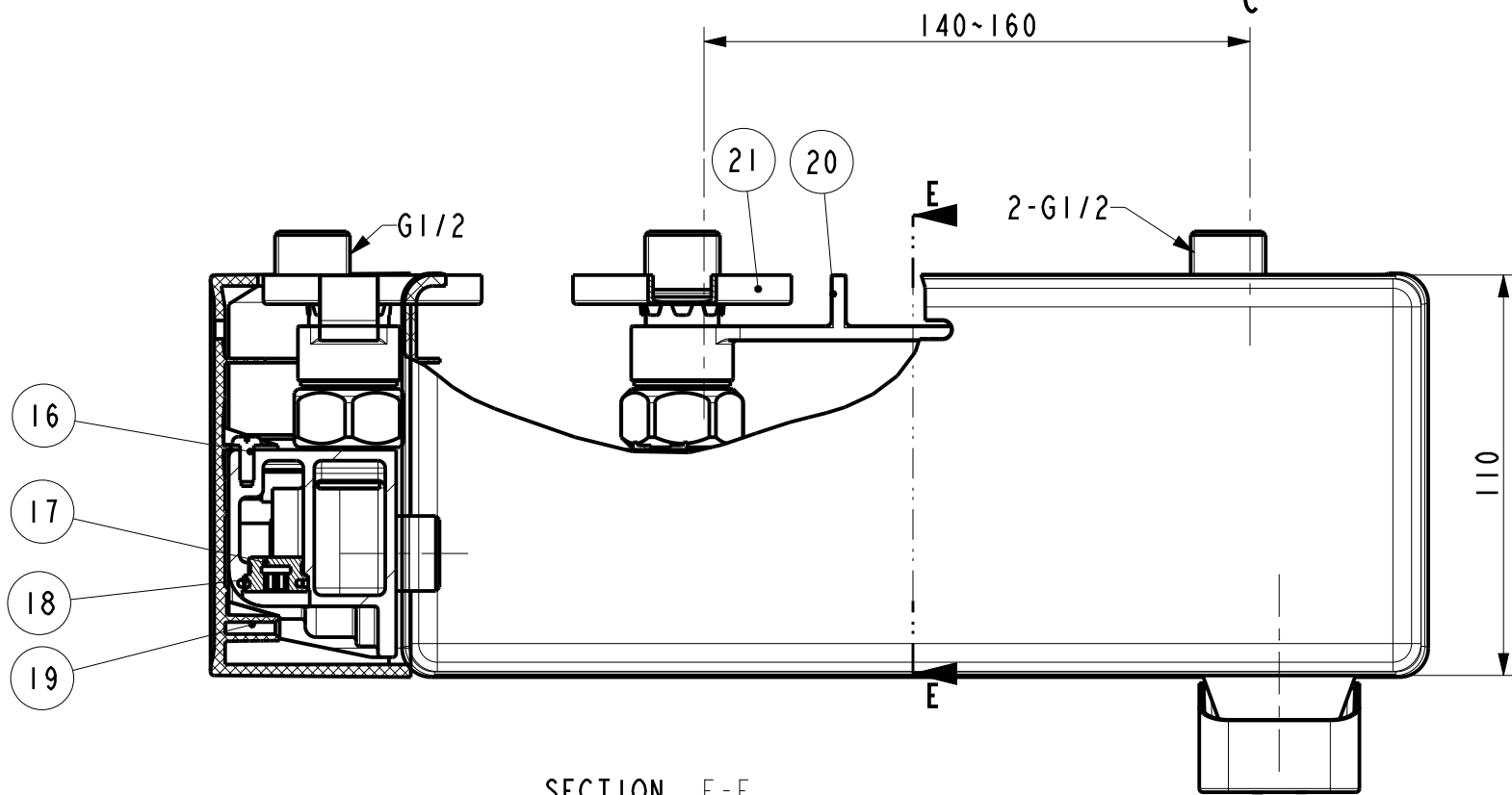
SECTION E-E
